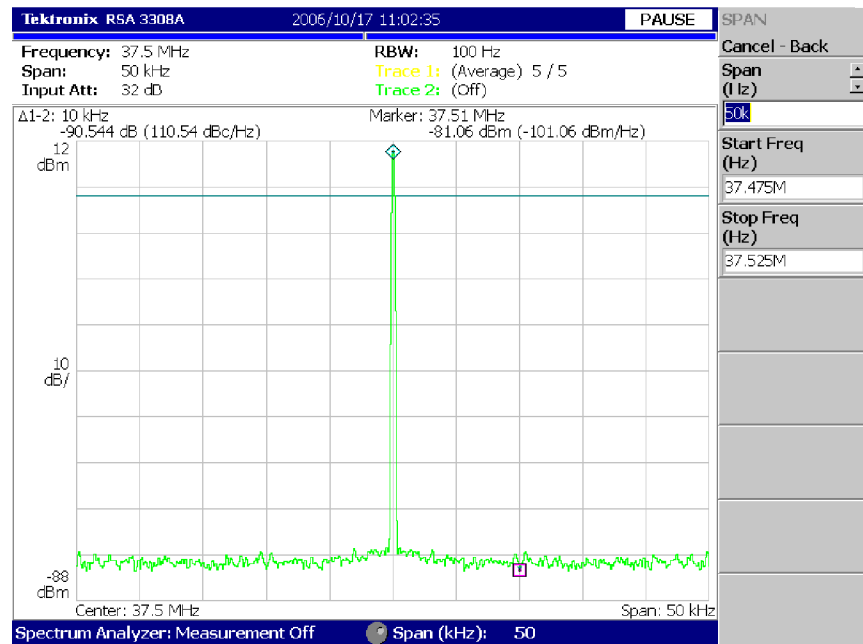
Figure 13: Example of the analog phase noise measurement
